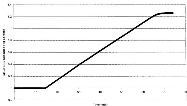
Figure 5. Amount of \text{CO}_2 adsorption from 15% \text{CO}_2 , 82% \text{N}_2 , 3% \text{O}_2 (saturated with water) mixture as a function of time on zeolite 1.
