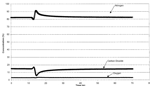
Figure 8. Adsorption of \text{CO}_2 , \text{N}_2 , and \text{O}_2 on zeolite 3 in atmospheric reactor at 25 °C (15% \text{CO}_2 , 3% \text{O}_2 , 82% \text{N}_2 and saturated with water vapor).
