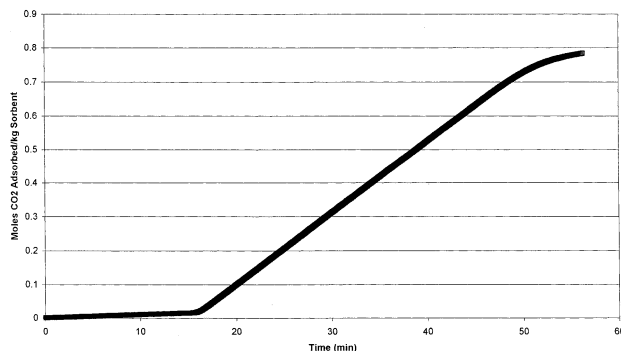
Figure 7. Amount of \text{CO}_2 adsorption from 15% \text{CO}_2 , 82% \text{N}_2 , 3% \text{O}_2 (saturated with water) mixture as a function of time on zeolite 2.
