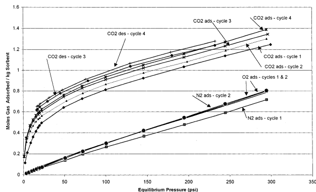
Figure 2. Adsorption and desorption isotherms of zeolite 2.
