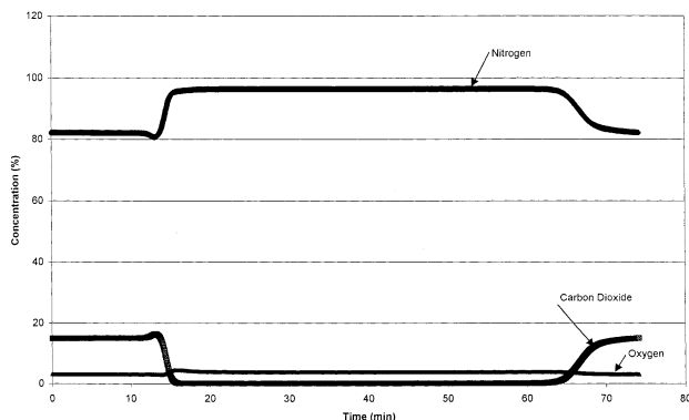
Figure 4. Adsorption of \text{CO}_2 , \text{N}_2 , and \text{O}_2 on zeolite 1 in atmospheric reactor at 25 °C (15% \text{CO}_2 , 3% \text{O}_2 , 82% \text{N}_2 and saturated with water vapor).
