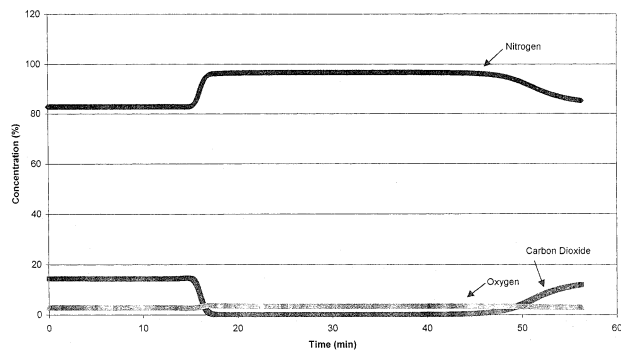
Figure 6. Adsorption of \text{CO}_2 , \text{N}_2 , and \text{O}_2 on zeolite 2 in atmospheric reactor at 25 °C (15% \text{CO}_2 , 3% \text{O}_2 , 82% \text{N}_2 and saturated with water vapor).
